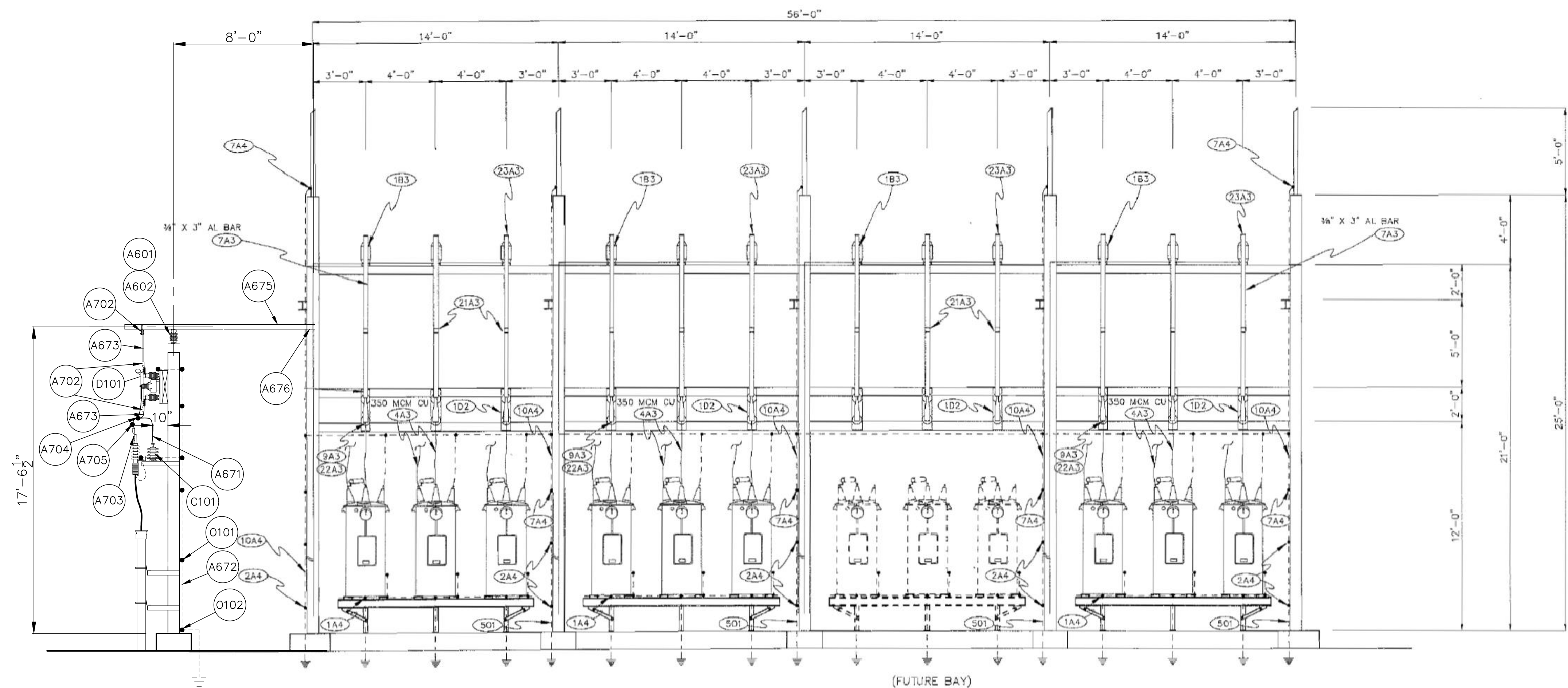
SECTION H-H
