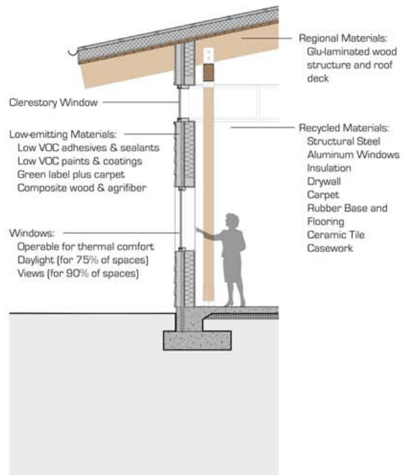
Section at Classroom
