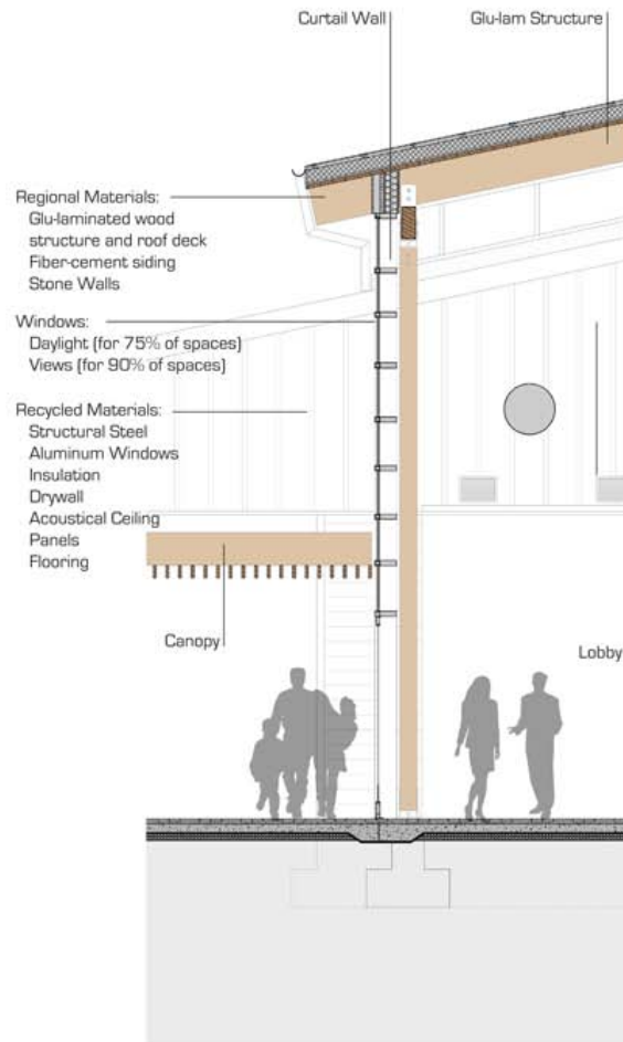
Section at Entrance Lobby
