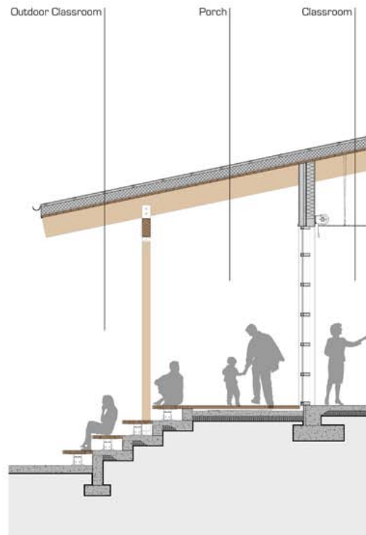
Section at Outdoor Classroom
