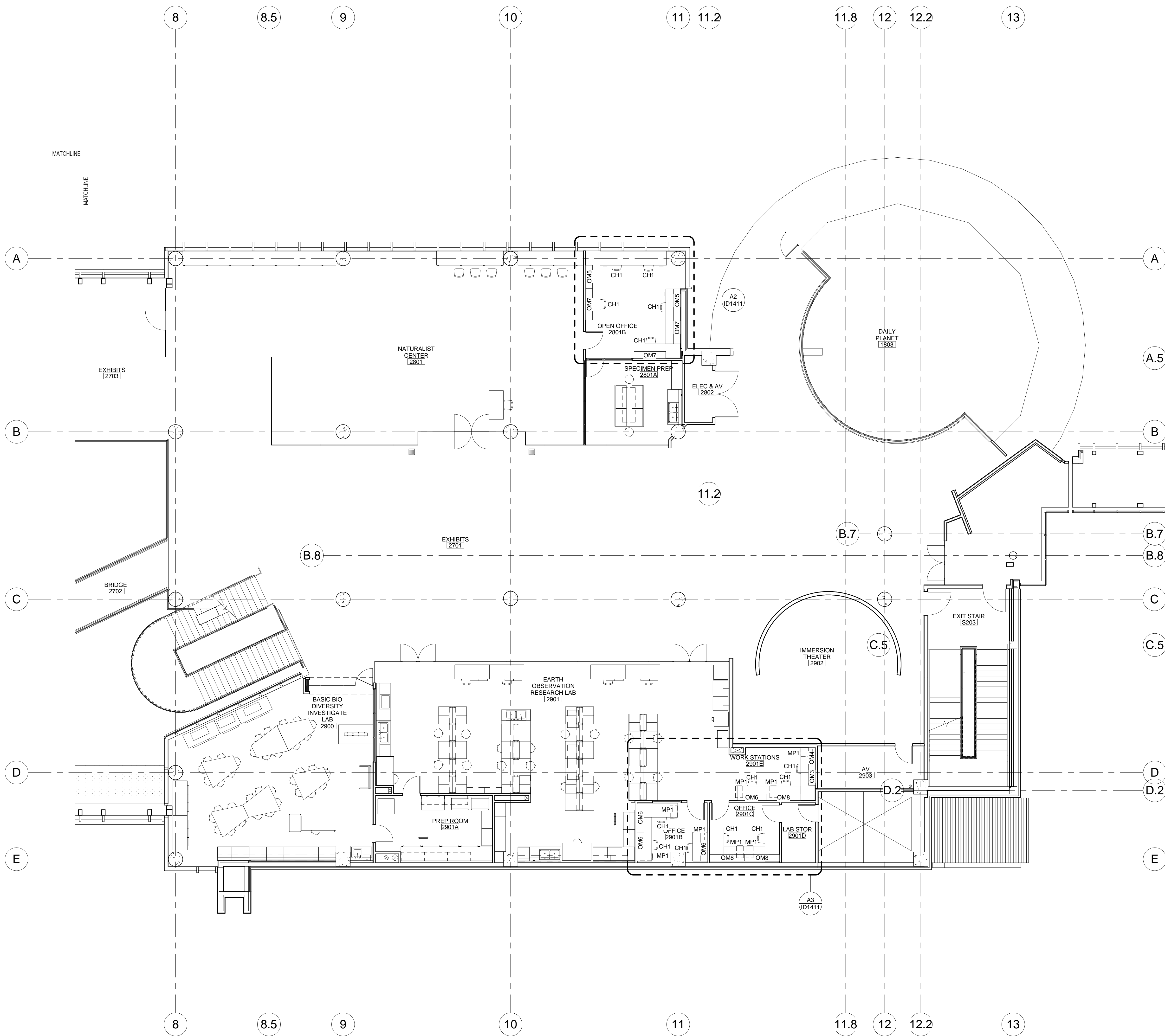
1 LEVEL TWO FURNITURE PLAN - AREA 2 ID1322 1/8" = 1'-0"
