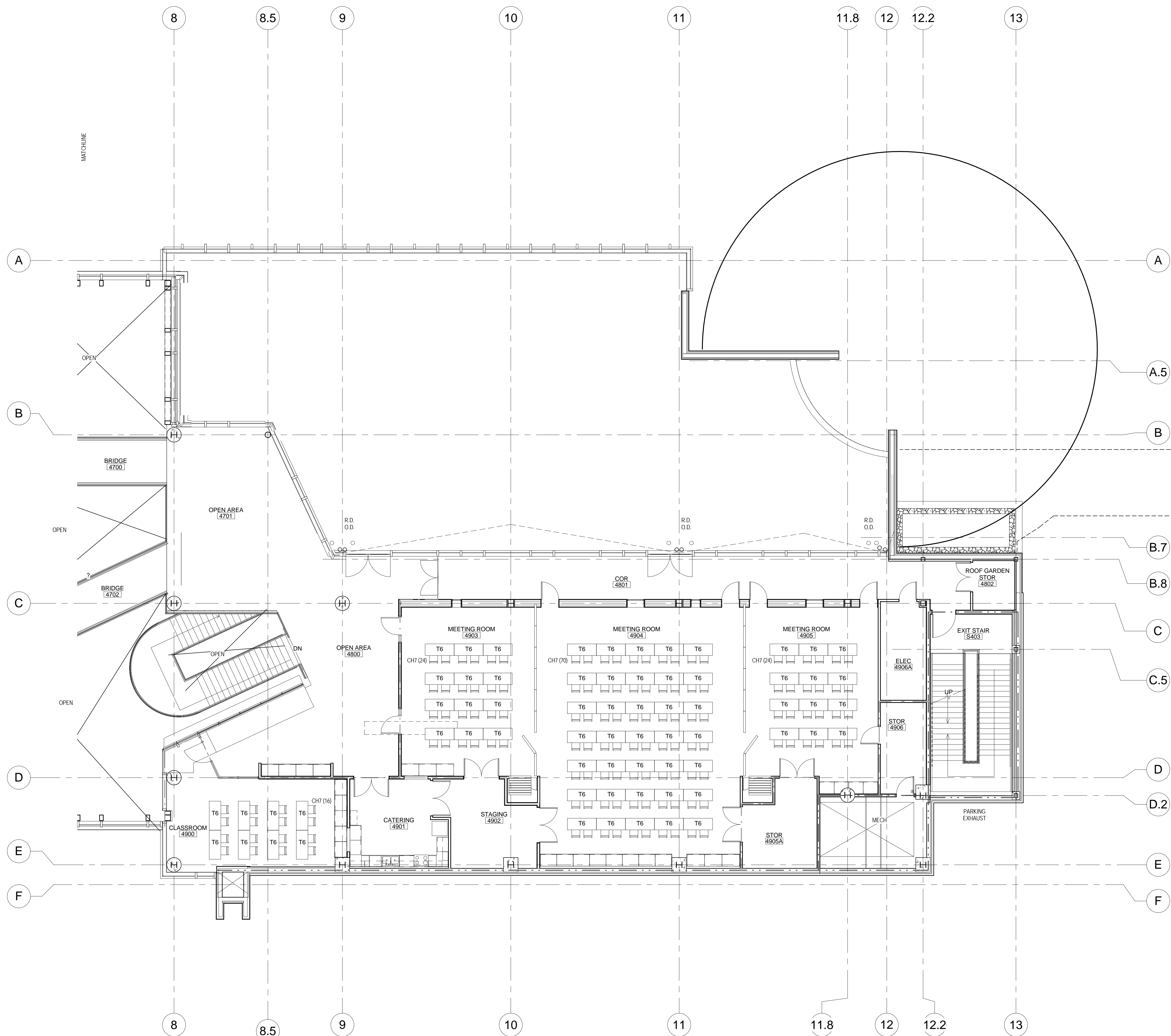
1 LEVEL FOUR FURNITURE PLAN - AREA 2 ID1342 1/8" = 1'-0"
